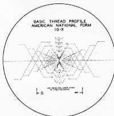
THREAD CHART
