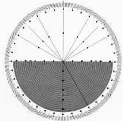
TWO-QUADRANT PROTRACTOR
